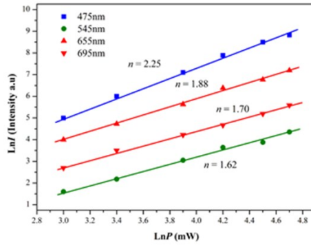
Fig. 4 : Logarithmic scale dependence of the UC emission intensity on the pump power in the range from 20 to 110 mW at 475, 545, 655 and 695 nm in the KY_{0.50}(WO_4)_2:Ho_{0.02}/Yb_{0.45}/Tm_{0.03} sample.
