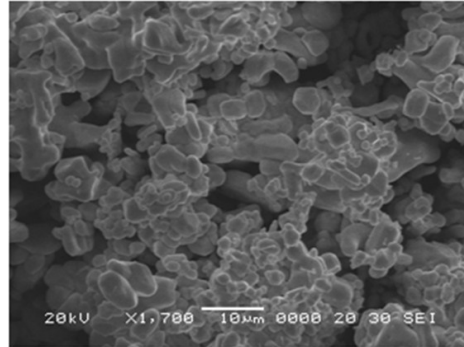
Fig. 2: SEM images of the synthesized \text{KY}_{0.50}(\text{WO}_4)_2:\text{Ho}_{0.02}/\text{Yb}_{0.45}/\text{Tm}_{0.03} particles.
