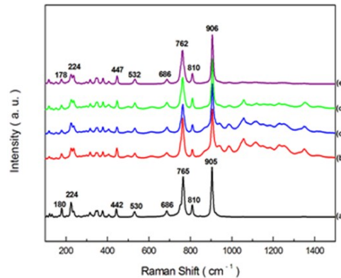
Fig. 6: Raman spectra of the synthesized (a) pure KYW (b) \text{KY}_{0.60}(\text{WO}_4)_2:\text{Ho}_{0.04}/\text{Yb}_{0.35}/\text{Tm}_{0.01} , (c) \text{KY}_{0.55}(\text{WO}_4)_2:\text{Ho}_{0.03}/\text{Yb}_{0.40}/\text{Tm}_{0.02} , (d) \text{KY}_{0.50}(\text{WO}_4)_2:\text{Ho}_{0.02}/\text{Yb}_{0.45}/\text{Tm}_{0.03} , and (e) \text{KGd}_{0.45}(\text{WO}_4)_2:\text{Ho}_{0.01}/\text{Yb}_{0.50}/\text{Tm}_{0.04} particles excited by the 514.5-nm line of an Ar ion laser at 0.5 mW.
