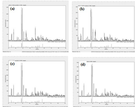
Fig. 1: XRD patterns of the synthesized (a) KY_{0.60}(WO_4)_2:Ho_{0.04}/Yb_{0.35}/Tm_{0.01} , (b) KY_{0.55}(WO_4)_2:Ho_{0.03}/Yb_{0.40}/Tm_{0.02} , (c) KY_{0.50}(WO_4)_2:Ho_{0.02}/Yb_{0.45}/Tm_{0.03} , and (d) KY_{0.45}(WO_4)_2:Ho_{0.01}/Yb_{0.50}/Tm_{0.04} particles.
