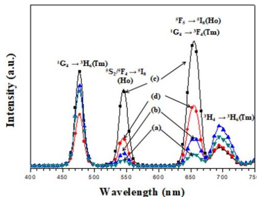
Fig. 3: UC PL emission spectra of (a) \text{KY}_{0.60}(\text{WO}_4)_2:\text{Ho}_{0.04}/\text{Yb}_{0.35}/\text{Tm}_{0.01} , (b) \text{KY}_{0.55}(\text{WO}_4)_2:\text{Ho}_{0.03}/\text{Yb}_{0.40}/\text{Tm}_{0.02} , (c) \text{KY}_{0.50}(\text{WO}_4)_2:\text{Ho}_{0.02}/\text{Yb}_{0.45}/\text{Tm}_{0.03} and (d) \text{KY}_{0.45}(\text{WO}_4)_2:\text{Ho}_{0.01}/\text{Yb}_{0.50}/\text{Tm}_{0.04} particles excited under 980 nm at room temperature.
